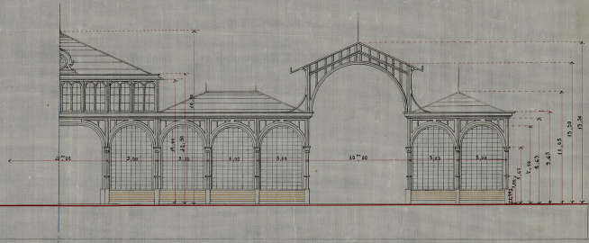
Fachada principal
